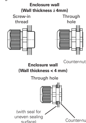
Fig. 3 Mounting in
