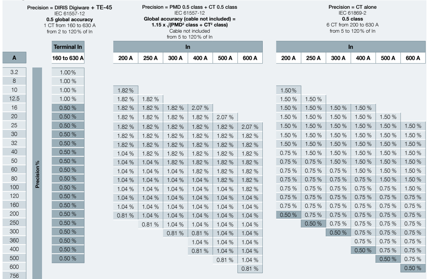
Fig. 13 - Comparing the accuracy achieved by DIRIS Digiware and PMD+CT from 160 to 630 A.
