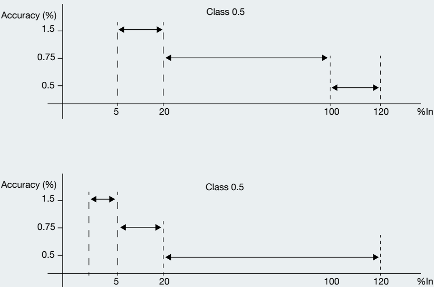
Fig. 1 - Difference between a standard and a s-class transformer.
