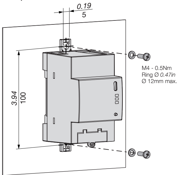
Back plate
