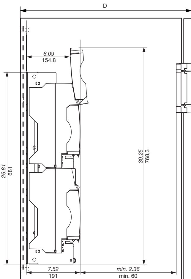
Side view
