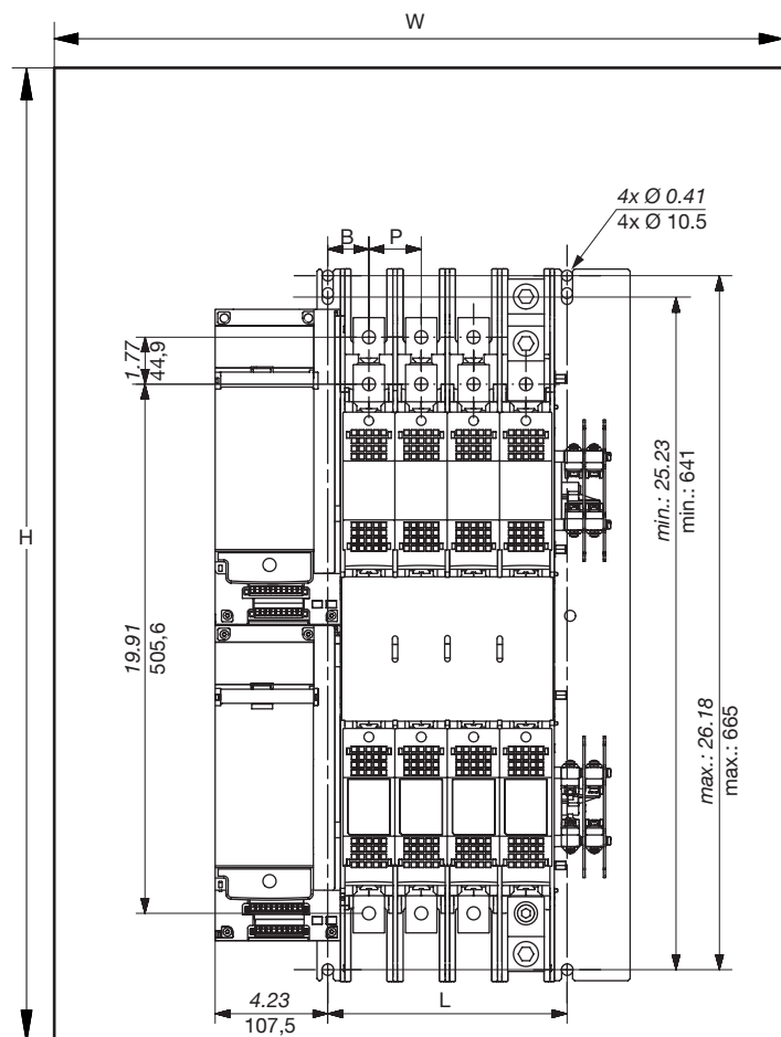
Front view
