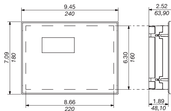
Controller dimensions
